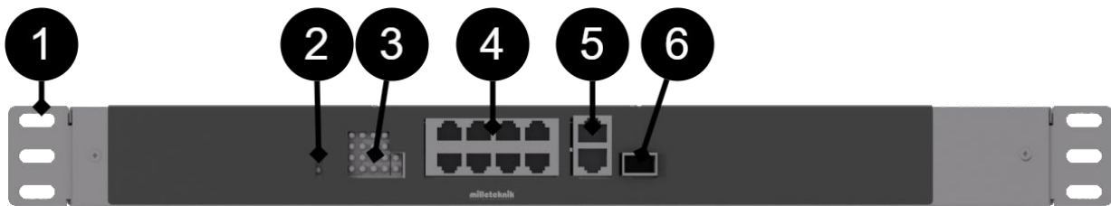
Component Overview PoE Switch 8p managed 1HE
